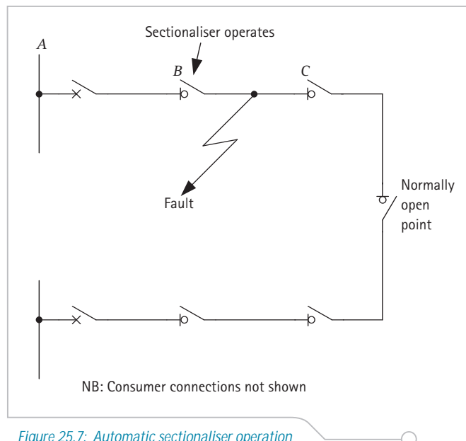
Figure 25.7: Automatic sectionaliser operation
