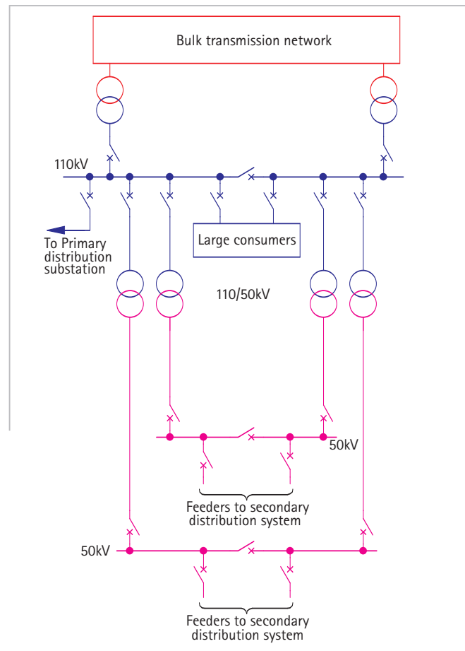
Figure 25.2: Primary distribution system
