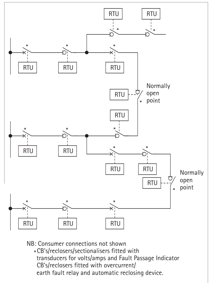
Figure 25.9: Automated rural distribution network
