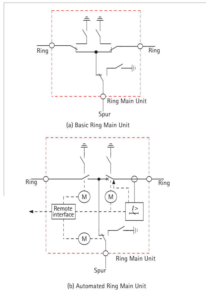
Figure 25.4: Ring Main Unit
